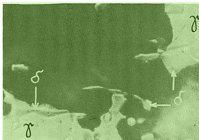
FIGURE 8 — Pit growth in quenched austenitic-ferritic steel, \gamma -phase undergoes corrosion, whereas \delta -phase remains unattacked. 10
