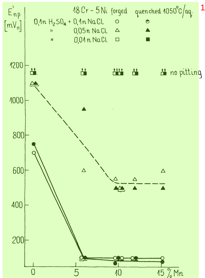
FIGURE 5 — Effect of Mn content on potential of pit nucleation. 2
