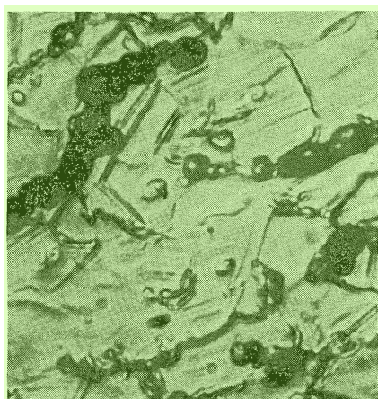
FIGURE 6 — Typical micrograph of forged steel after corrosion. 1600X 4
